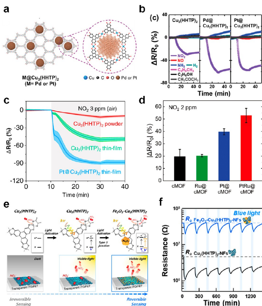
Figure 10. (a) Schematic illustration for nanoparticle encapsulation of \text{Cu}_3(\text{HHTP})_2 (b) Selective gas sensing performance of \text{Cu}_3(\text{HHTP})_2 , \text{Pd}@ \text{Cu}_3(\text{HHTP})_2 , and \text{Pt}@ \text{Cu}_3(\text{HHTP})_2 . Reprinted with permission under a Creative Commons CC BY License from ref 120. Copyright 2019 Wiley-VCH. (c) Sensing performance for \text{Cu}_3(\text{HHTP})_2 powder, thin film, and thin film with Pt decoration using microfluidic channel-embedded solution shearing. Reprinted with permission under a Creative Commons CC BY License from ref 104. Copyright 2021 Springer Nature. (d) Sensing responses of Pt, Ru, and PtRu NP- encapsulated \text{Cu}_3(\text{HHTP})_2 for 2 ppm of \text{NO}_2 . Reprinted with permission from ref 122. Copyright 2021 Wiley-VCH. (e) Reversible \text{NO}_2 sensing mechanism of \text{Fe}_2\text{O}_3-\text{Cu}_3(\text{HHTP})_2 using visible light. (f) Repetitive sensing traces of \text{Fe}_2\text{O}_3-\text{Cu}_3(\text{HHTP})_2 and \text{Cu}_3(\text{HHTP})_2 toward 5 ppm of \text{NO}_2 under blue light illumination. Reprinted with permission under a Creative Commons CC BY-NC-ND License from ref 99. Copyright 2021 American Chemical Society.
