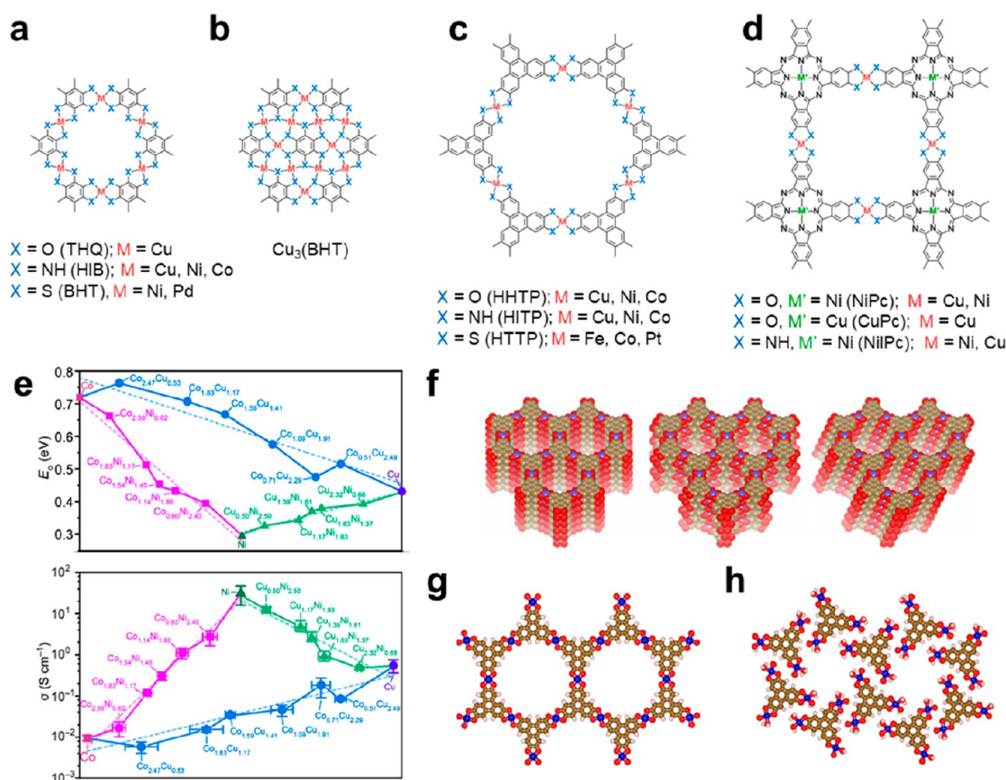
Figure 2. Structure of lattice layers in (a) benzene-based 2D c-MOFs, (b) Cu 3 (BHT), (c) triphenylene-based 2D c-MOFs, and (d) phthalocyanine-based 2D c-MOFs. (e) Variation in bandgaps and conductivities of M 3 (HITP) 2 with Co, Cu, and Ni nodes. Reprinted with permission from ref 88. Copyright 2020 American Chemical Society. (f) Possible stacking arrangements (eclipsed, serrated, and inclined) of 2D layers. Structures of (g) extended frameworks and (h) discrete complexes.
