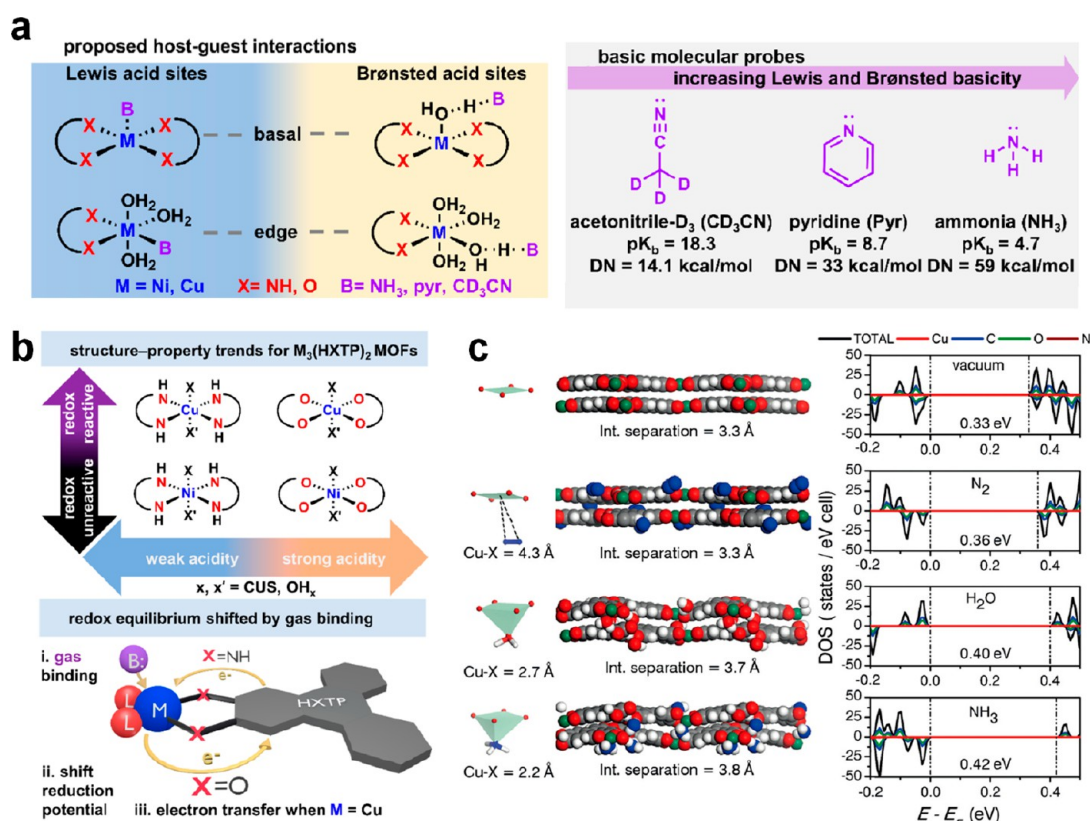
Figure 3. (a) Possible interactions of metal nodes in M_3(\text{HHTP})_2 and M_3(\text{HITP})_2 ( M = \text{Cu} and \text{Ni} ) with basic molecular probes. (b) The trend in redox activities and acidities of M_3(\text{HHTP})_2 and M_3(\text{HITP})_2 . Adapted with permission from ref 95. Copyright 2020 American Chemical Society. (c) DFT-optimized structures and density of states of \text{Cu}_3(\text{HHTP})_2 interacting with \text{N}_2 , \text{H}_2\text{O} , and \text{NH}_3 . Reprinted with permission from ref 94. Copyright 2019 Wiley-VCH.
