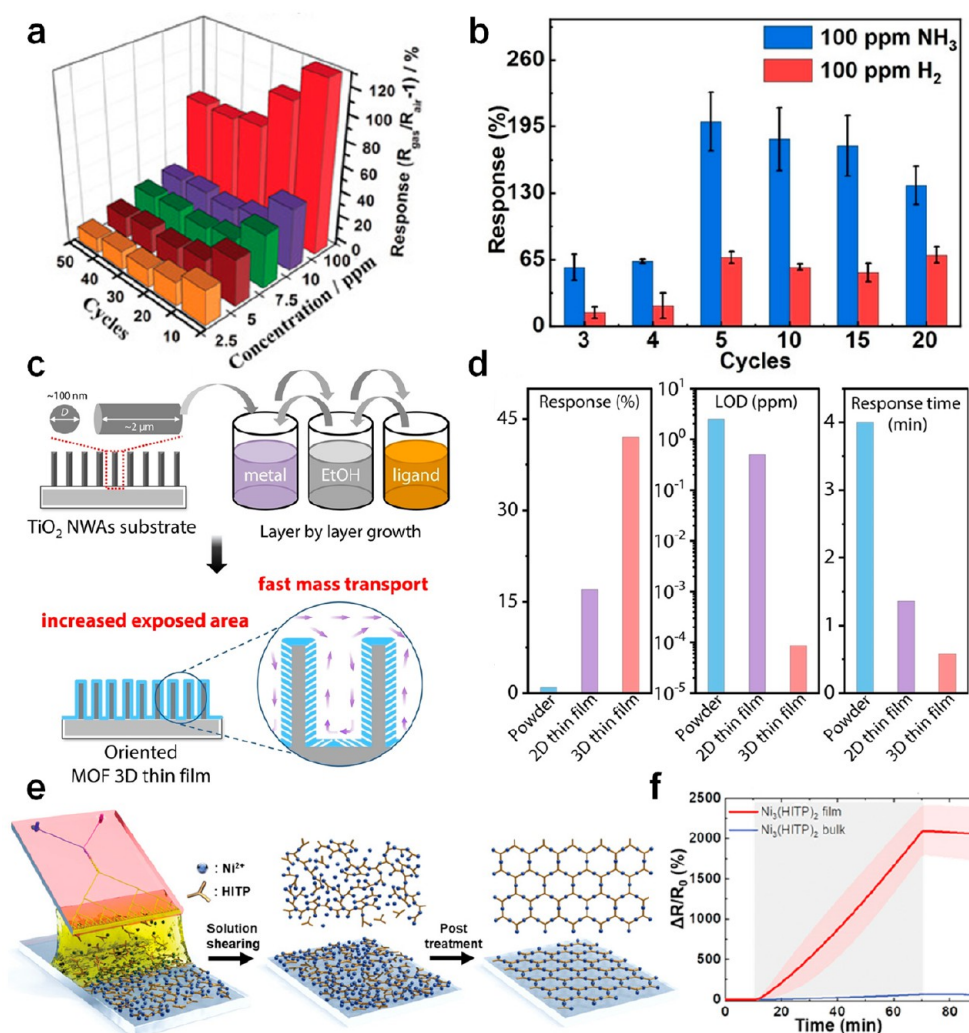
Figure 9. (a) \text{NH}_3 sensing responses of \text{Cu}_3(\text{HHTP})_2 film with different LBL growth cycles. Reprinted with permission from ref 98. Copyright 2017 Wiley-VCH. (b) Growth-cycle-dependent responses of the \text{Cu}_3(\text{HHTP})_2 film toward 100 ppm of \text{NH}_3 and \text{H}_2 . Reprinted with permission from ref 113. Copyright 2022 Wiley-VCH. (c) Schematic illustration for fabrication of oriented MOF 3D thin film using the LBL assembly technique. (d) Sensing performance for powder, 2D thin film, and 3D thin film of \text{Cu}_3(\text{HHTP})_2 . Reprinted with permission from ref 114. Copyright 2021 Wiley-VCH. (e) The schematic figure for fabrication of \text{Ni}_3(\text{HITP})_2 thin-film processing using the microfluidic-based solution shearing (f) Dynamic sensing trace of bulk and thin-film \text{Ni}_3(\text{HITP})_2 toward 5 ppm of \text{H}_2\text{S} . Reprinted with permission from ref 115. Copyright 2022 Wiley-VCH.
